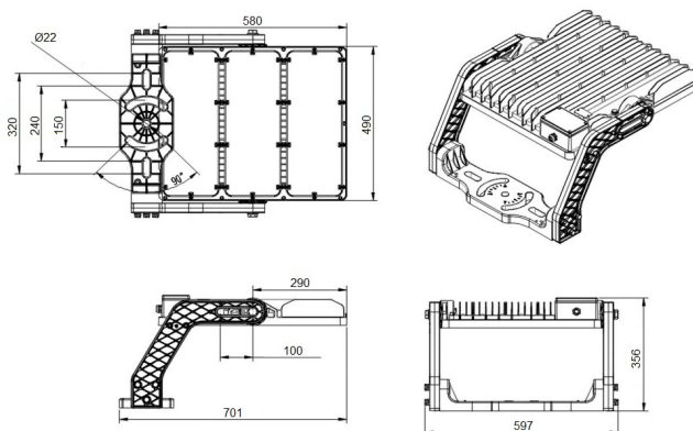
1000/1200W LED module
