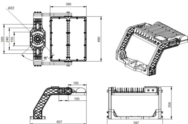
600/800W LED module
